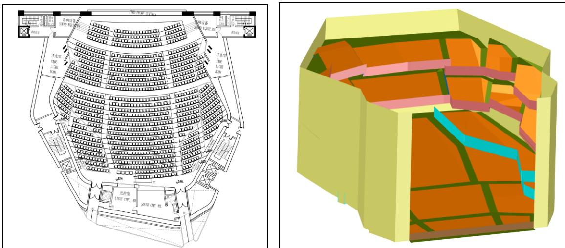
Figure 2: Plan and first 3d model of the Opera House
