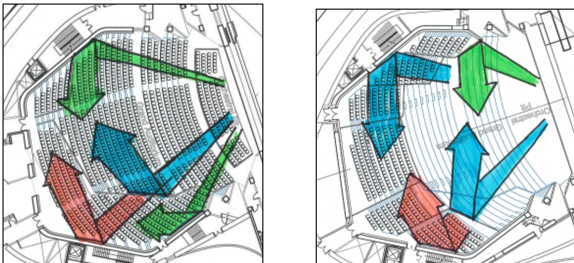
Figure 3: Scheme for distributing first order reflections in the Opera House
